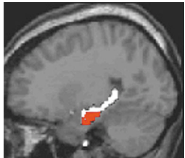
FIGURE 4. T1-weighted structural image for a single subject is shown with the hippocampal ROI superimposed on it. Voxels with significant susceptibility-induced signal loss (T2* signals that were below the intensity threshold to detect activation [ITDA]) are shown in red. Note that in this subject (and in 8 of 11 other subjects), such voxels were found only in the anterior half of the hippocampus. Within the anterior hippocampus, such voxels were located inferiorly, closest to the skull base and sinuses, further suggesting that this signal loss is caused by susceptibility artifact.
